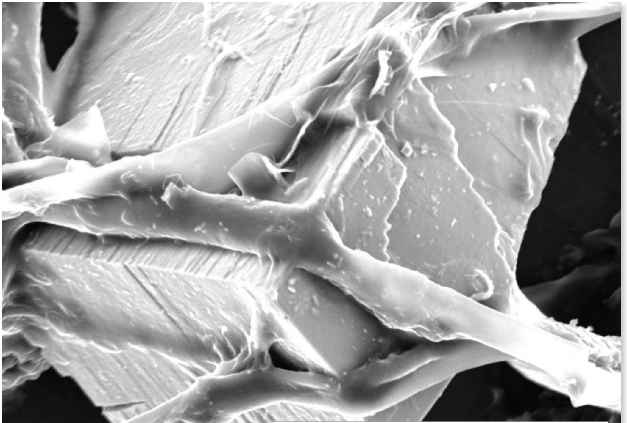
Fig. 4.6: Fungi attacking a crystal of Galena (PbS). Observe the mode of attachment of fungal hyphae to mineral surface at 90°. (KK)
